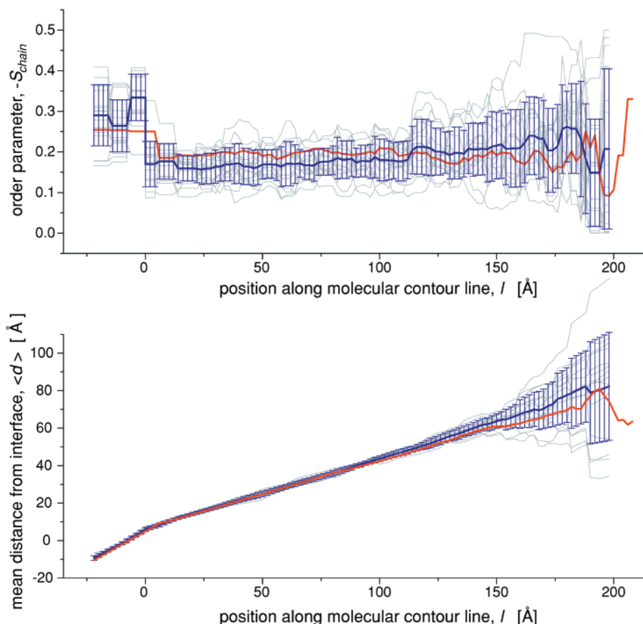
Figure 3. (a) Chain order parameter, S_{chain} , determined according to eq 4 and (b) mean distances, \langle d \rangle , from the aqueous surface of subsections located at distances l along the contour line of the polymer chains for the synthetic (red) and recovered (blue) configuration sets shown in Figure 2; negative l values correspond to the alkyl chains. Thin gray lines indicate data of individual data inversion runs. Error bars give standard deviations of 16 independent runs.
